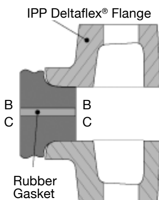
Fig.2 Steel Stub-end
